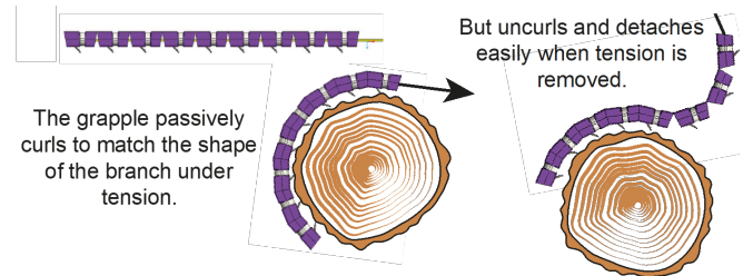
Fig. 6: The compliant grapple passively curls to the shape of the branch, engaging the microspines to distribute the load, while still being easily detachable - [25]©[2019] IEEE.
