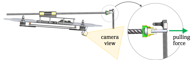
Fig. 2: Passively compliant mechanism for direct sensor placement.
