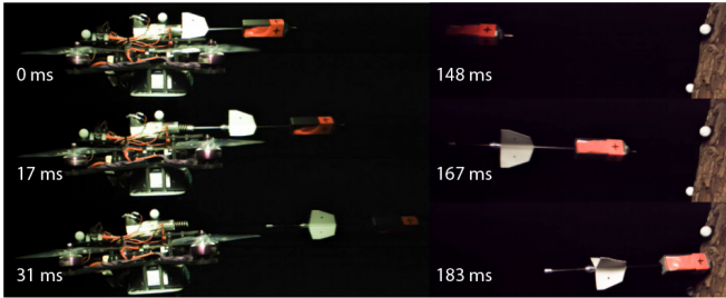
Fig. 10: Launching and impact sequence recorded at 1600 fps.
