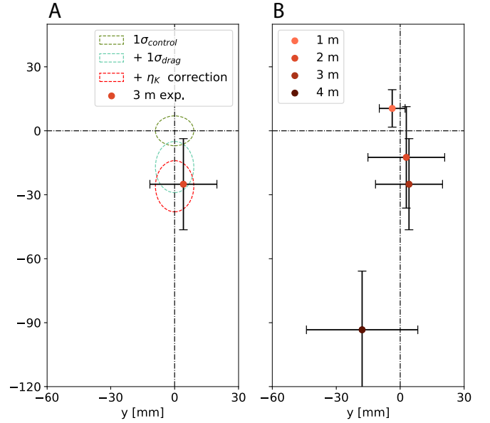
Fig. 9: Sensor placement results for 64 tests executed on a flat metallic surface. A : Effect of control loop, sensor projectile drag and losses in potential - kinetic energy conversion. B : Mean and standard deviation of sensor placement experiments at 1 to 4 metres distance from a flat metallic surface (figure adapted from [26]).
