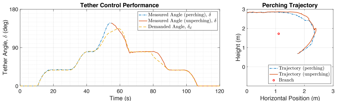
Fig. 7: Tensile perching experiment: motion tracking of the tether angle and the UAV's center-of-mass - [25]©[2019] IEEE.
